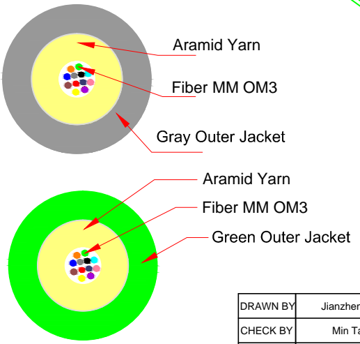
4. Cable structure
